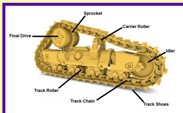
Undercarriage
